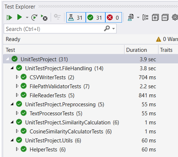
Fig 17: Unit Tests
